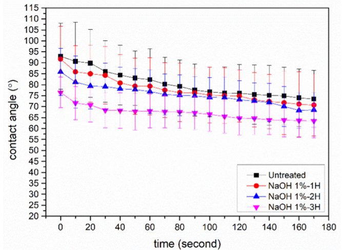
Figure 2 Measurement of PF contact angle to bamboo strand surfaces after 1% NaOH immersing treatment at 1, 2, and 3 hours, respectively, as a function of time
