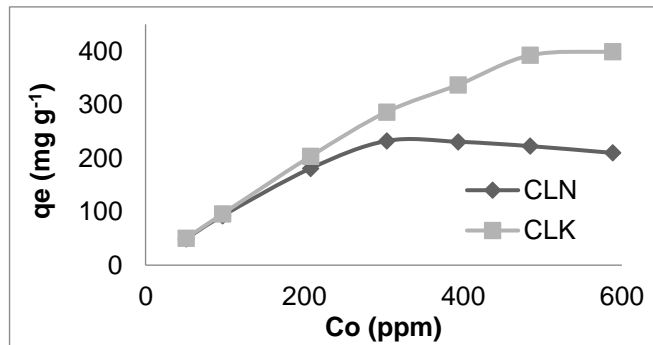
Figure 5. Effect of initial on sorption of MB by activated cassava leaves
