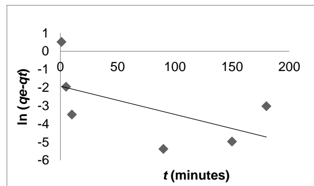
Figure 9. Pseudo-first-order model of MB sorption on CLK
