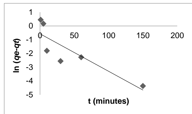
Figure 8. Pseudo-first-order model of MB sorption on CLN
