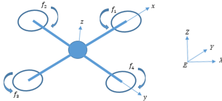
Fig. 1. Model of quadcopter
