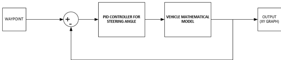
Figure 3. Diagram Block of Computer Simulation System
