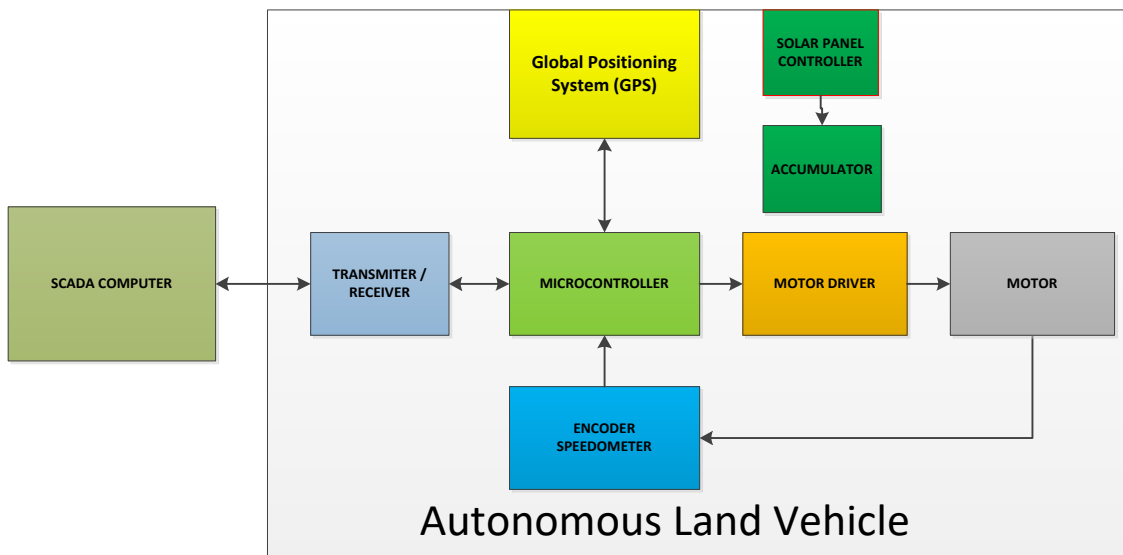
Figure 2. Diagram Block of Real Implementation System
