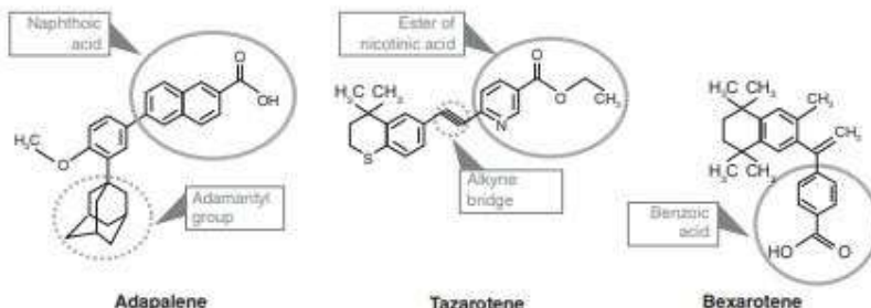
Figure 3. First, second, and third-generation retinoids (Williams et al. , 2020)
