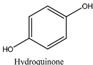
Figure 2. Chemical structure of hydroquinone (Andersen et al. , 2013)
